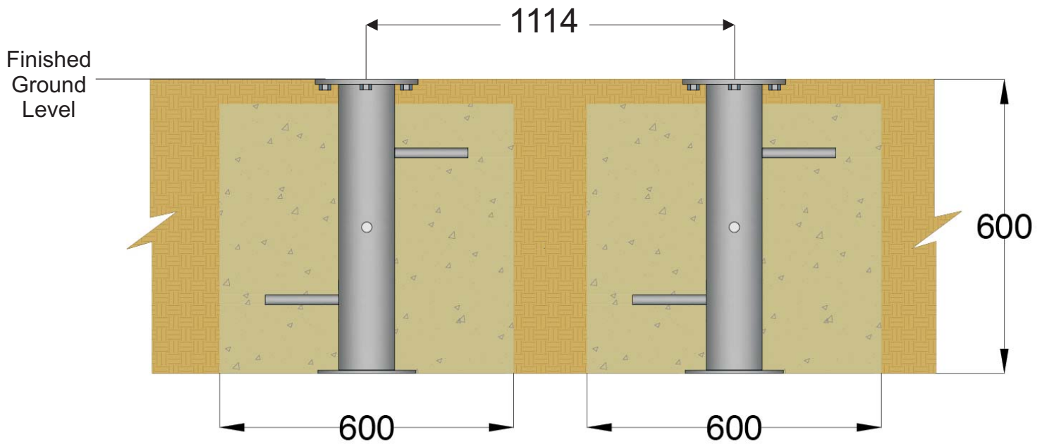
Foundation Detail(fig 1)
