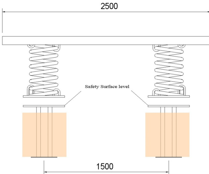
Foundation Detail (fig. 1) - Side Elevation
