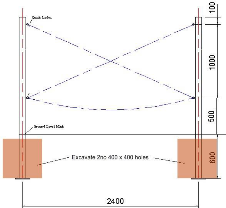
Foundation Detail (fig. 1) - Side Elevation
