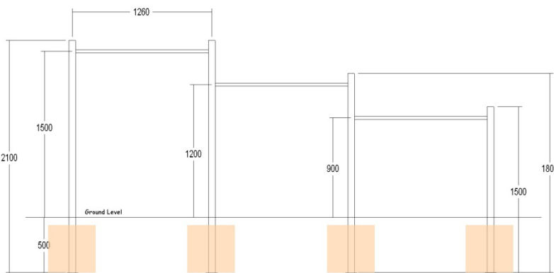
Foundation Detail (fig. 1) - Side Elevation
