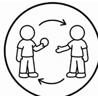
TURN-TAKING
